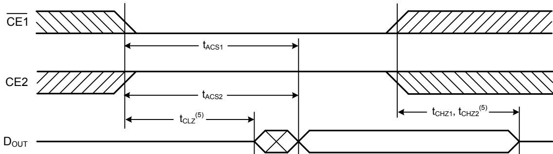
READ CYCLE 2 (1, 3, 4)
